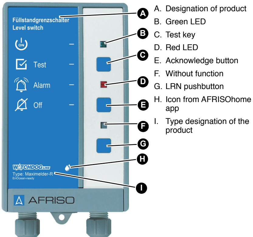
Fig 2: Control unit
