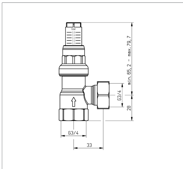
angled version
