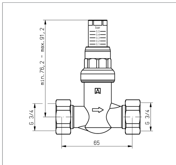
straight version
